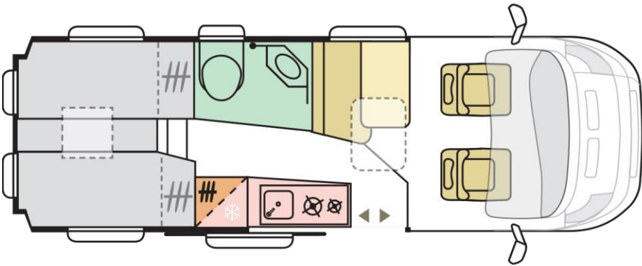
TWIN SUPREME 640 SGX
